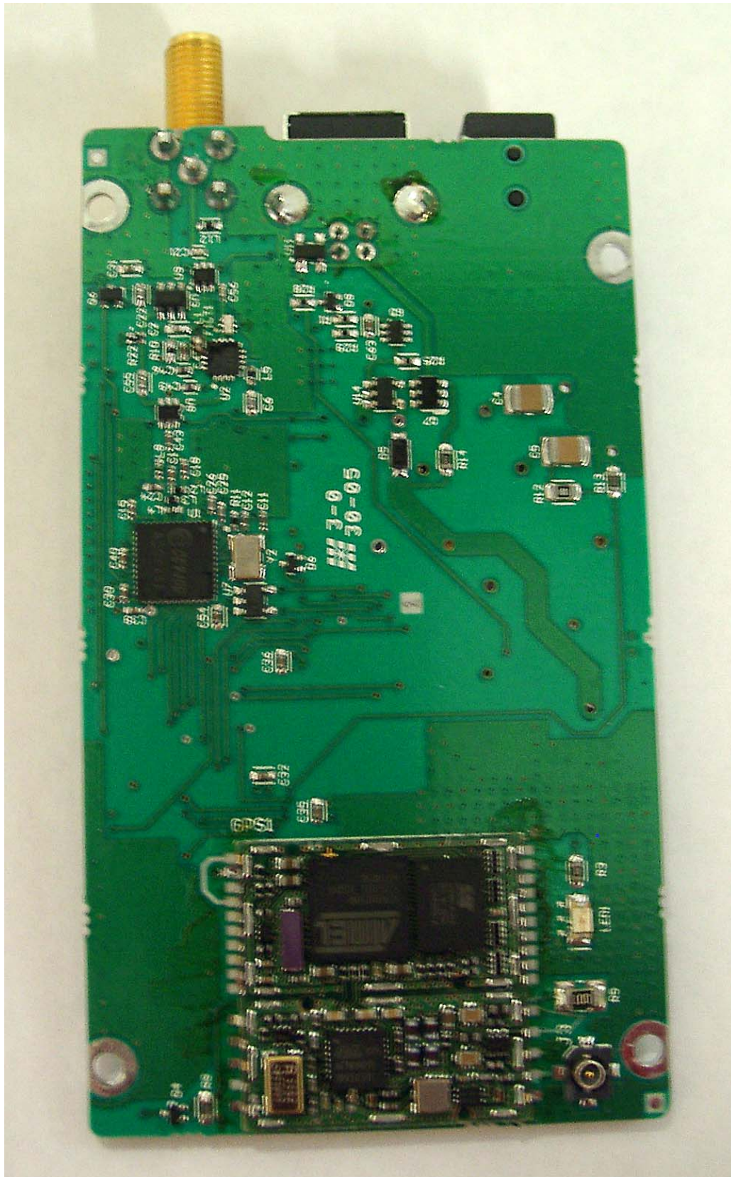
PCB Bottom Side
