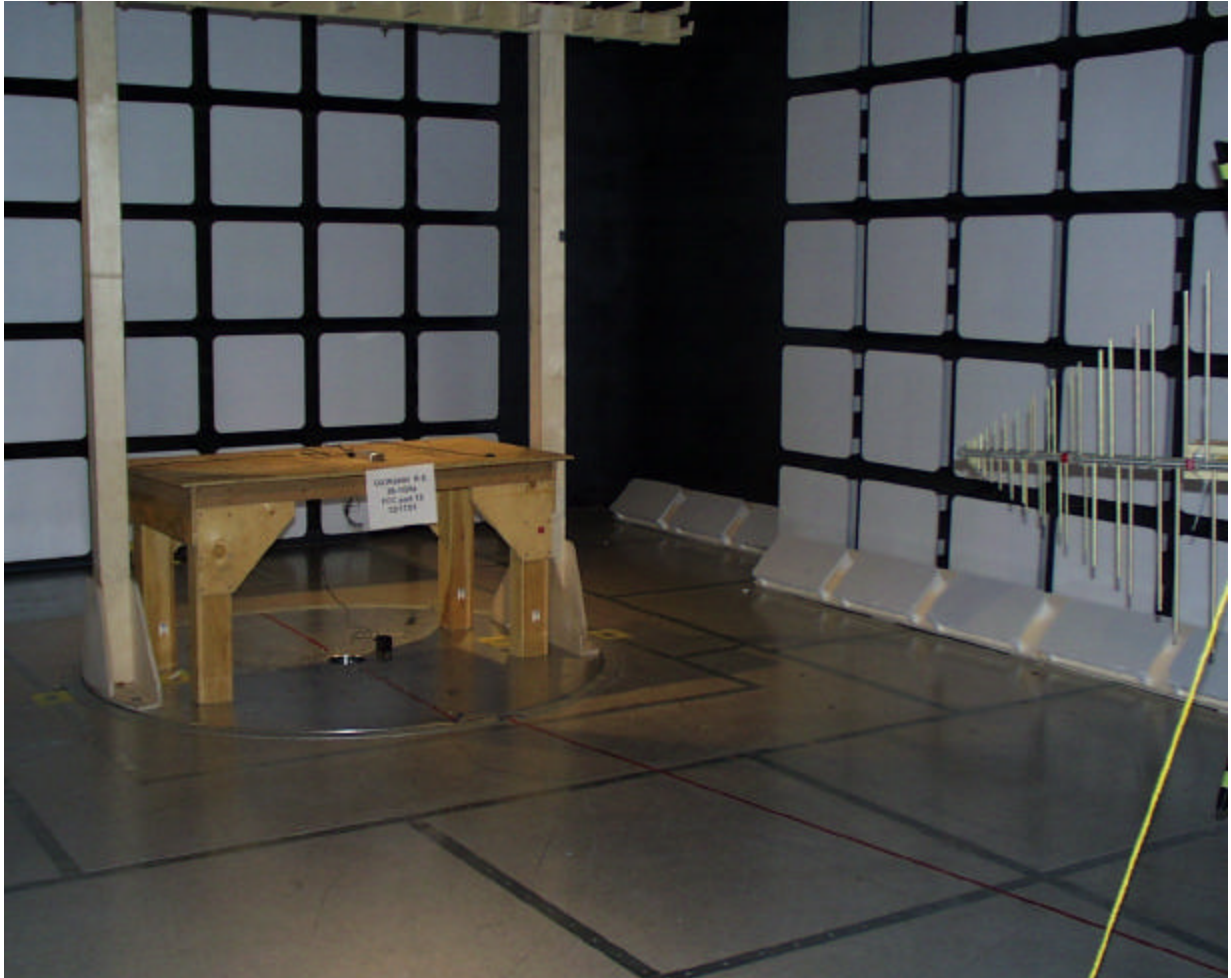
FCC Part 15 Emission setup
