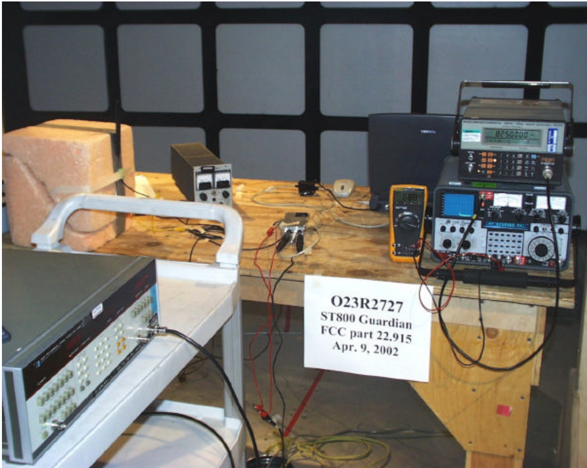
FCC Part 22.913 ERP measurement setup
