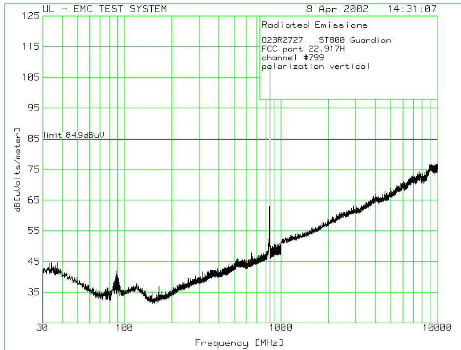
Part 22.917, Spurious emissions, channel CDMA # 799.
