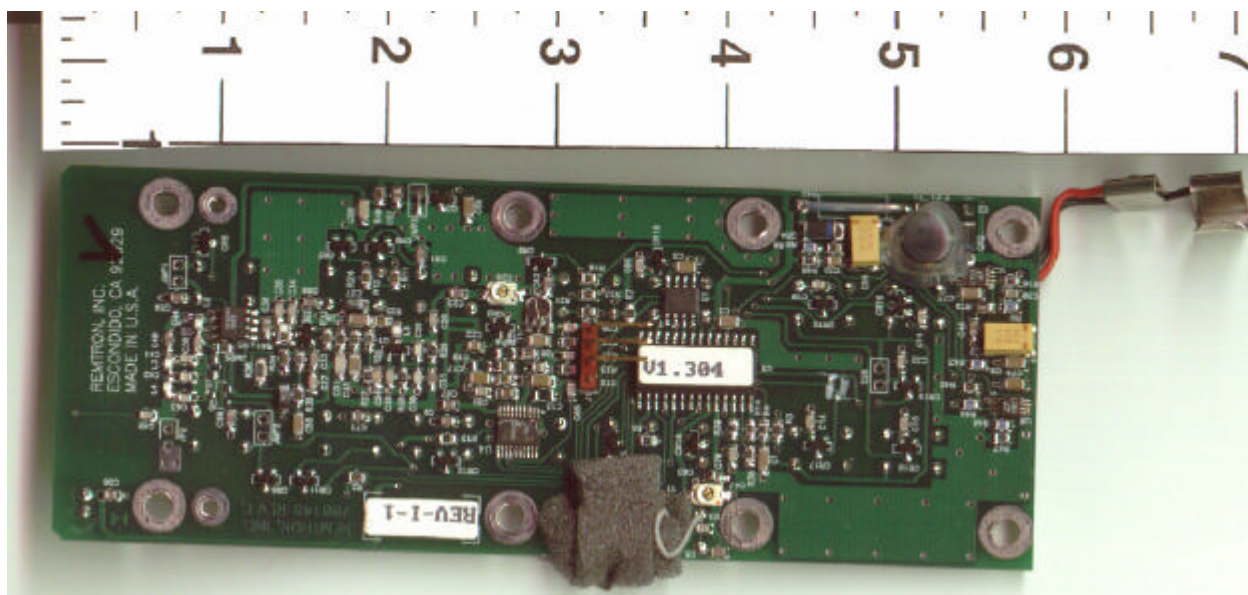
Front and Back of Low power transmitter 21T14 PCB
