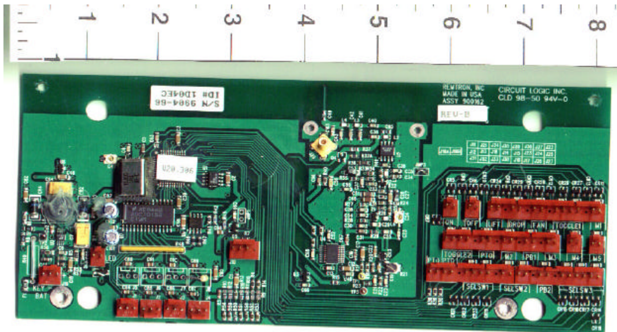
Front and Back of Belly Box Transmitter 21T34 PCB
