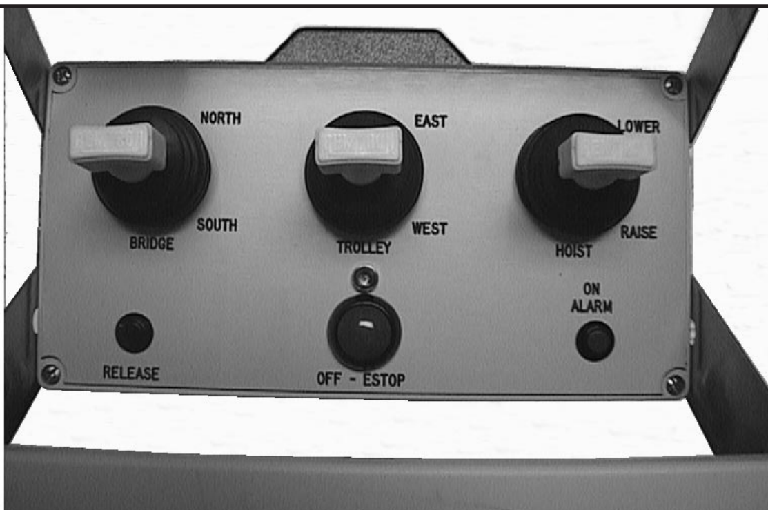
Figure 5.2 21T54 Transmitter
