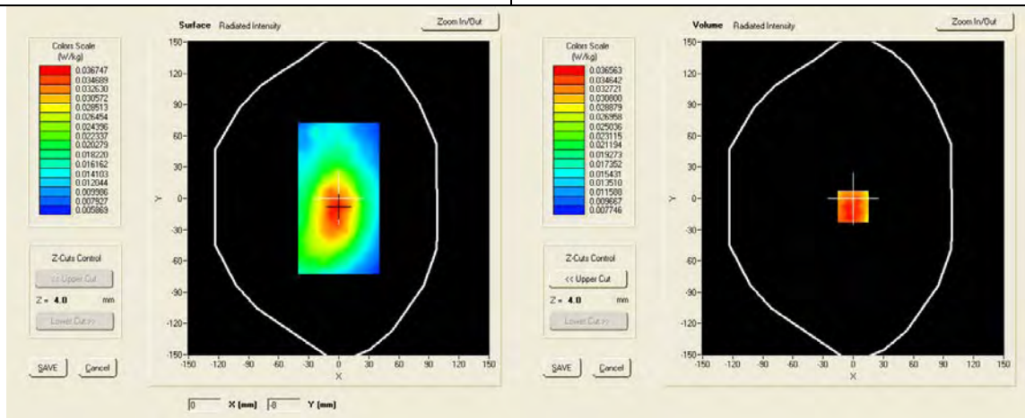
SAR, Z Axis Scan (X = 0, Y = -8)
