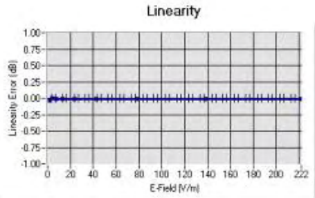
Linearity [±0.92% (±0.04dB)]
