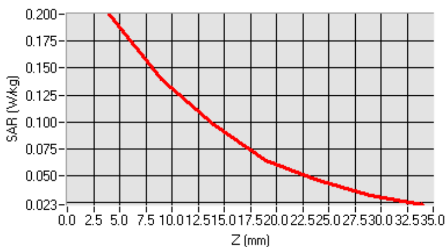
SAR, Z Axis Scan (X = 10, Y = -23)
