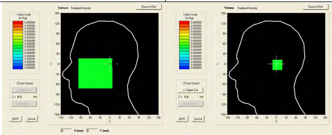
SAR, Z Axis Scan (X = 8, Y = -3)
