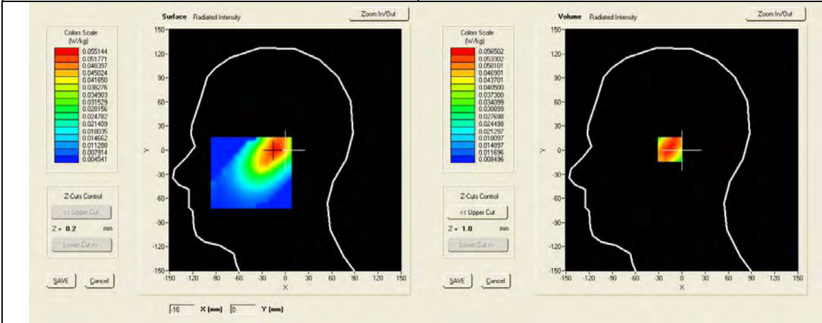
SAR, Z Axis Scan (X = -13, Y = 1)
