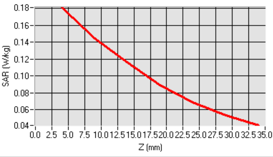
SAR, Z Axis Scan (X = -38, Y = -20)
