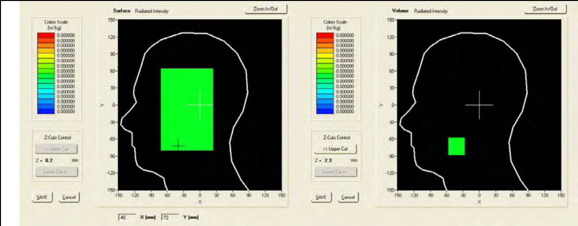
SAR, Z Axis Scan (X = -39, Y = -73)
