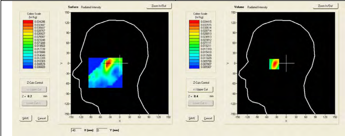
SAR, Z Axis Scan (X = -37, Y = -1)
