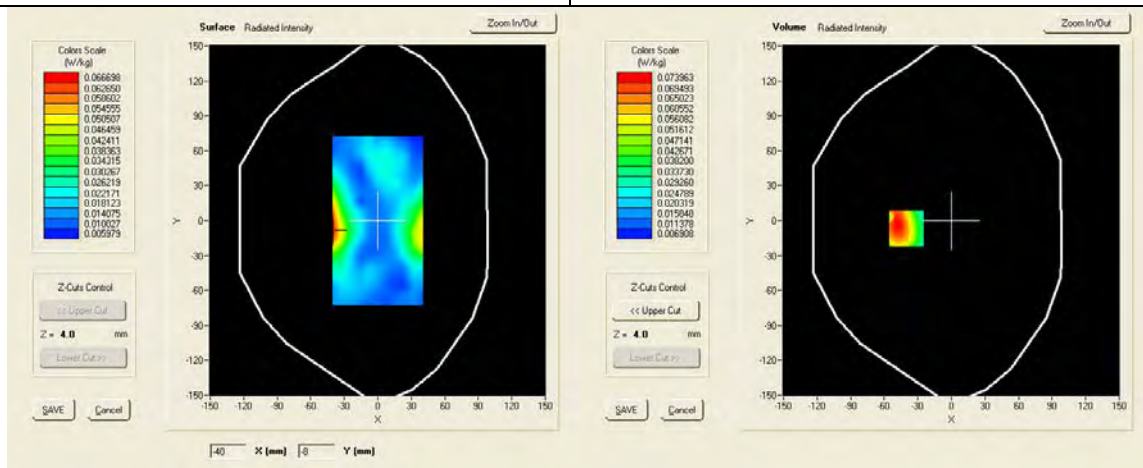
SAR, Z Axis Scan (X = -40, Y = -7)
