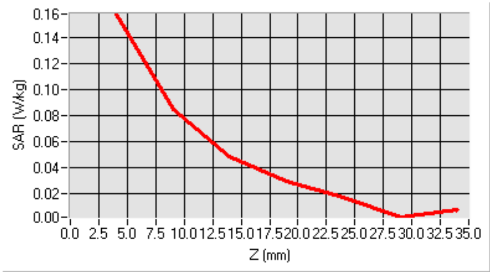
SAR, Z Axis Scan (X = 25, Y = -16)
