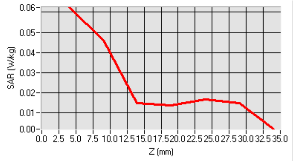
SAR, Z Axis Scan (X = 9, Y = 17)
