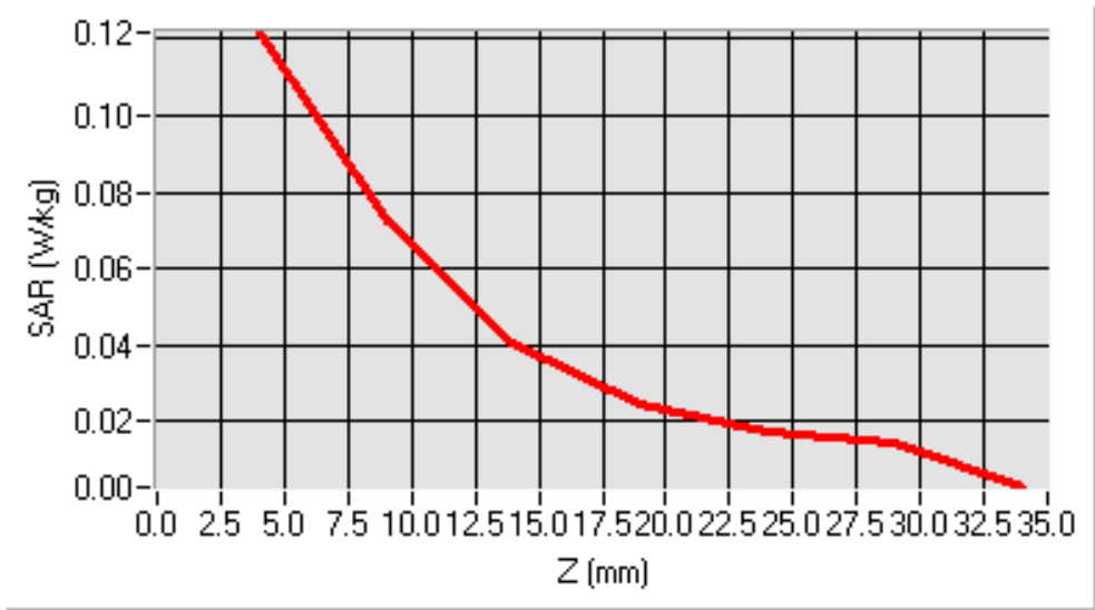
SAR, Z Axis Scan (X = 13, Y = 9)
