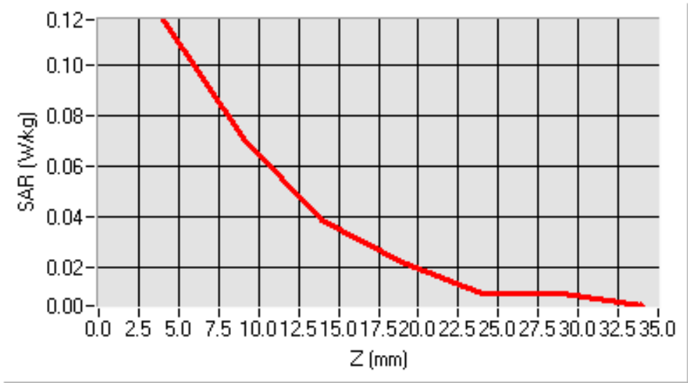
SAR, Z Axis Scan (X = 11, Y = 11)
