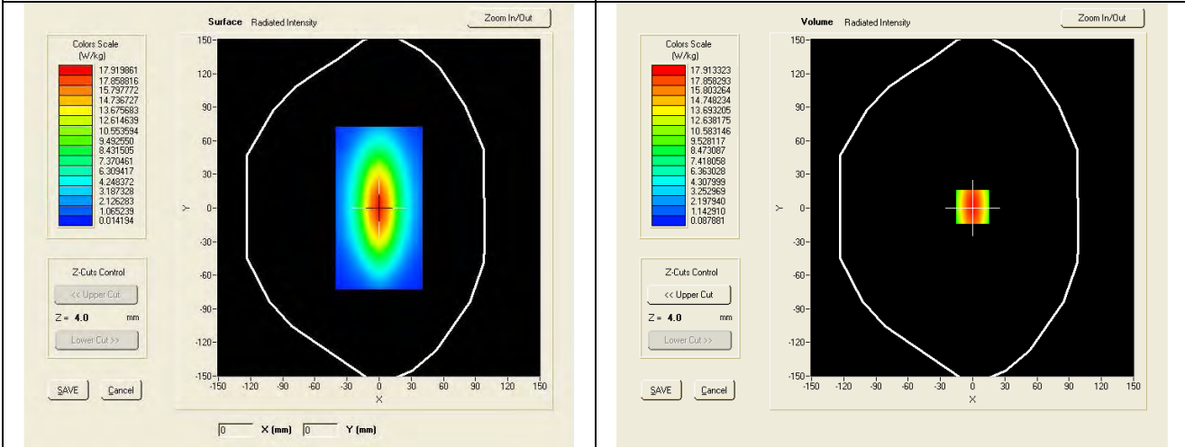
SAR, Z Axis Scan (X = 0, Y = 1)
