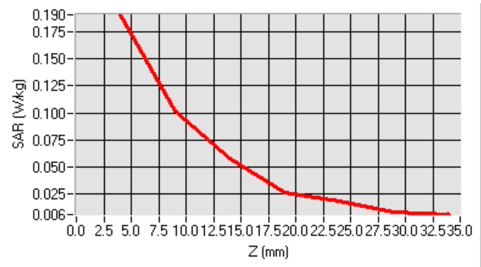
SAR, Z Axis Scan (X = 33, Y = -51)
