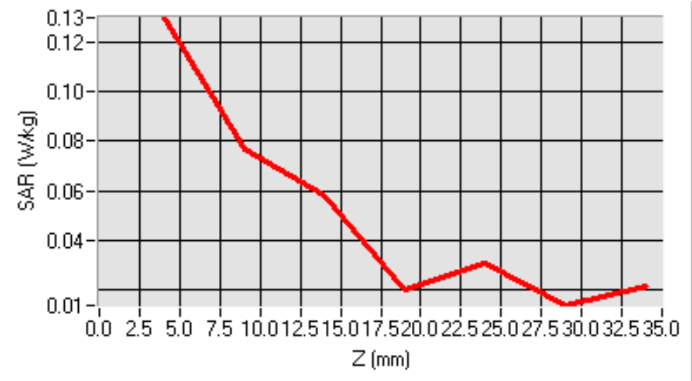
SAR, Z Axis Scan (X = 8, Y = -16)
