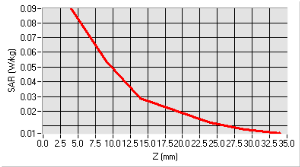
SAR, Z Axis Scan (X = 31, Y = -31)
