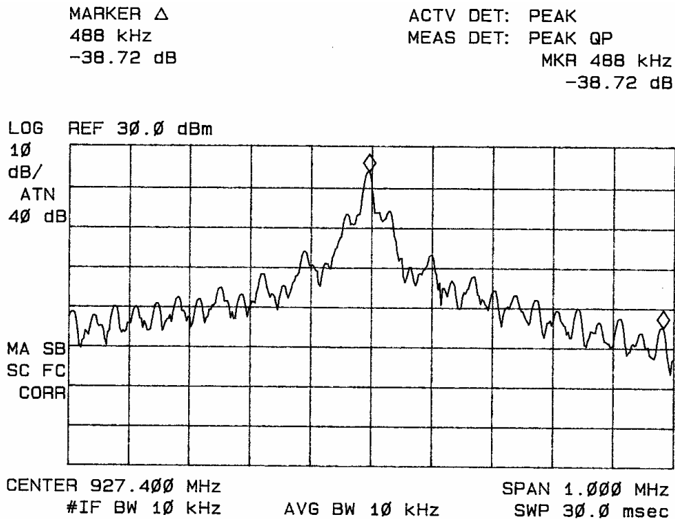
Figure 12. Band edge protection plot showing highest channel.
