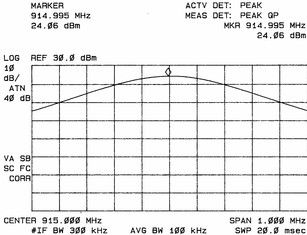
Figure 7. Maximum Power output.
