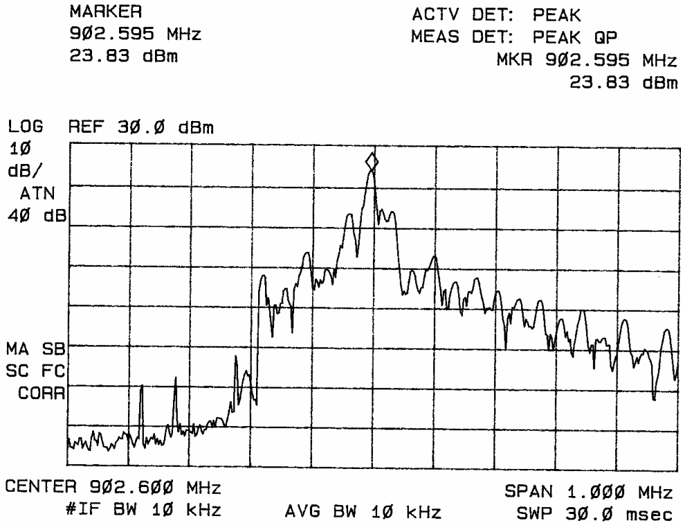
Figure 11. Band edge protection plot showing lowest channel.
