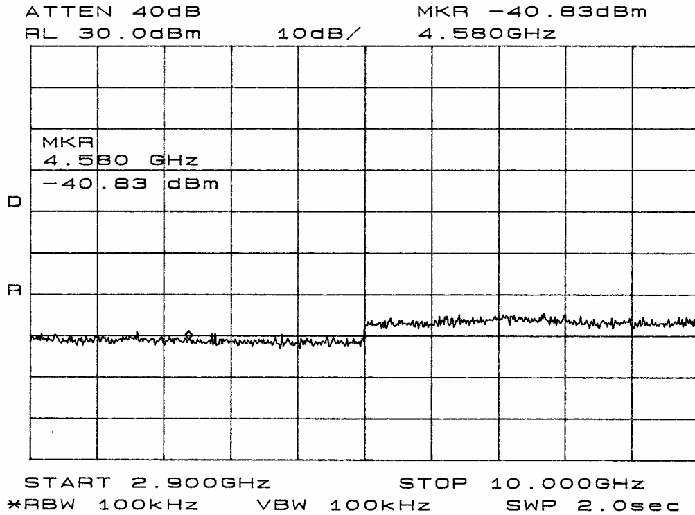
Figure 6. Antenna Conducted Emissions taken in the screen room.
