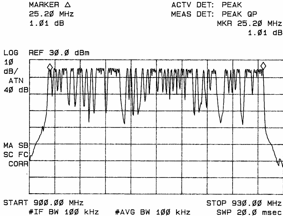
Figure 13. Full operational frequency band of 902928 MHz.
