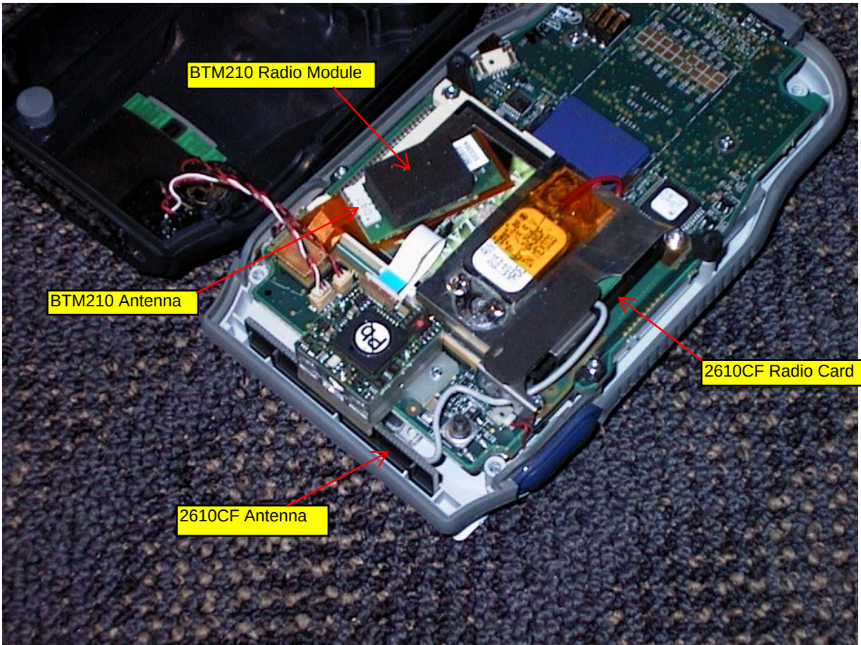
CN2B Radio/Antenna Placement
