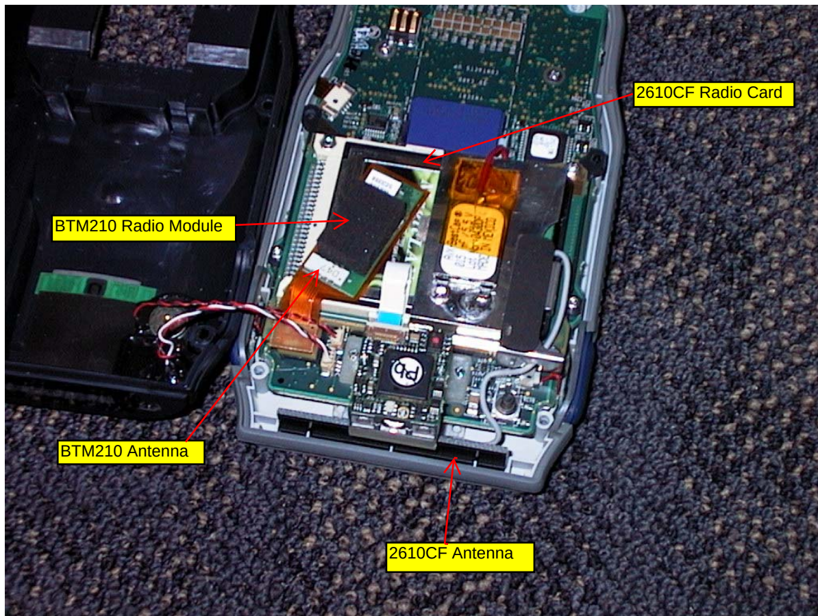
CN2B Unit Internal View
