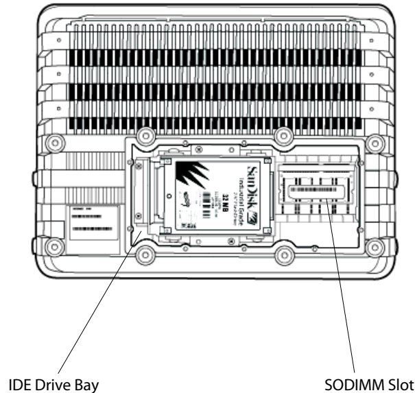
CV60 Rear View (Mounting Bracket Removed)
