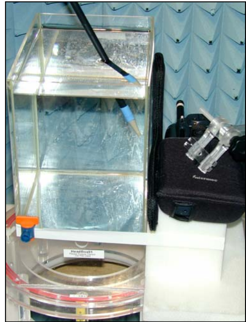
Figure 72. Positional photograph of the Intermec 700C Side (inverted) position holster 2
