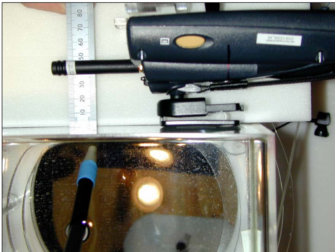
Figure 30. – Intermec 700C rear facing from phantom side representing use of belt clip
