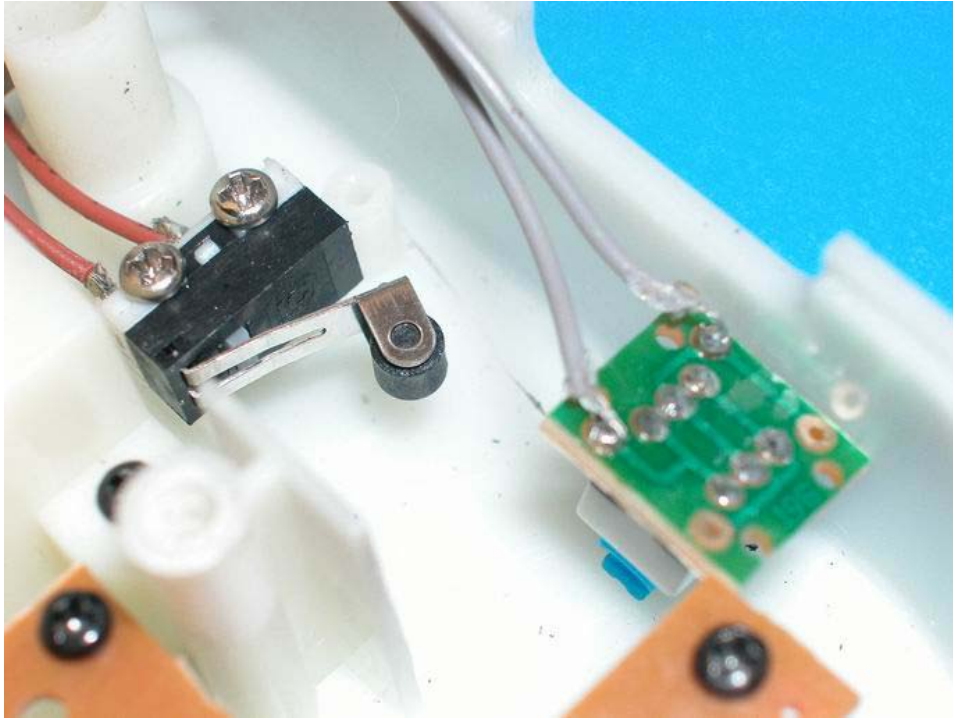
Internal Photo - 12
