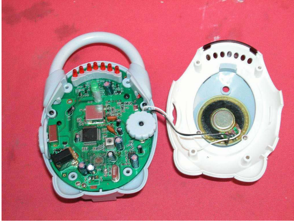
Assembly (View 1)
