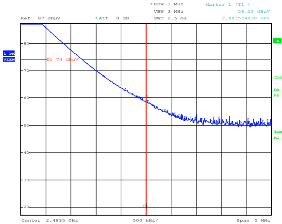
Figure 8.5-56: Radiated spurious emissions Upper band edge emission for BLE, High channel. F1 = 2.4835 GHz (beginning of restricted band)
