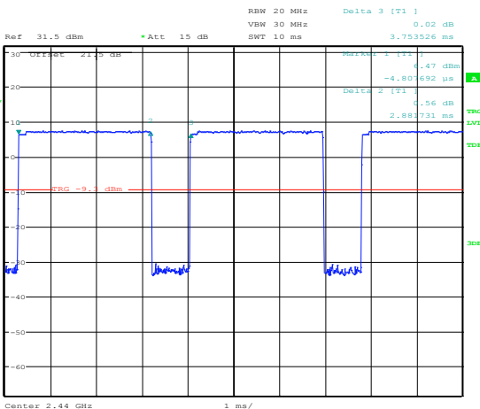
Figure 8.5-12: Pulse width for 2-DH3
