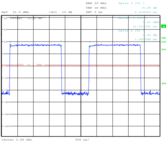
Figure 8.5-24: Pulse width for 3-EV3
