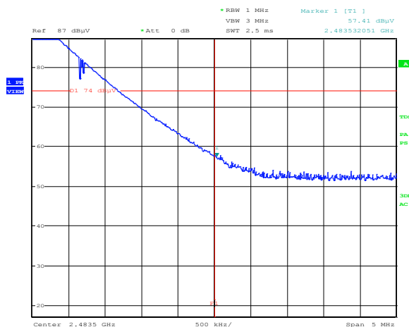
Figure 8.5-37: Radiated spurious emissions Upper band edge emission for BT, hopping is turned on. F1 = 2.4835 GHz (beginning of restricted band)
