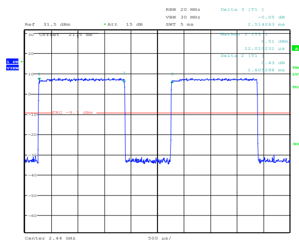
Figure 8.6-24: Pulse width for 3-EV3
