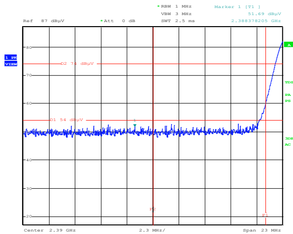
Figure 8.6-55: Radiated spurious emissions Lower band edge emission for BLE, low channel. F2 = 2.39 GHz (end of restricted band), F1 = 2.4 GHz
