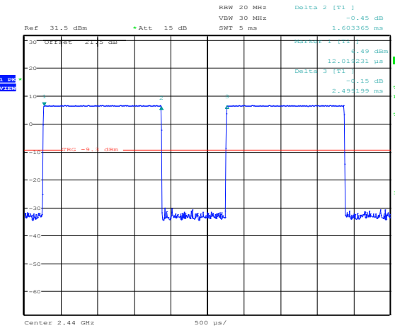
Figure 8.6-20: Pulse width for EV3
