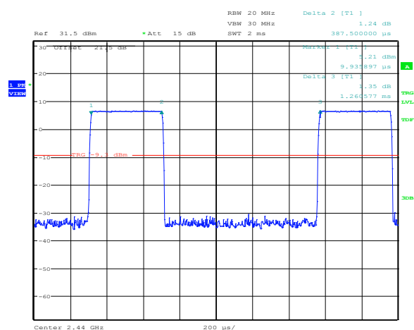
Figure 8.6-16: Pulse width for HV1
