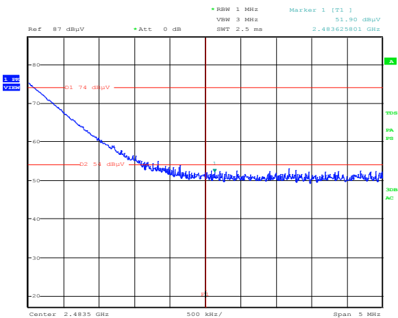
Figure 8.6-36: Radiated spurious emissions Upper band edge emission for BT, hopping is turned off – high channel. F1 = 2.4835 GHz (beginning of restricted band)
