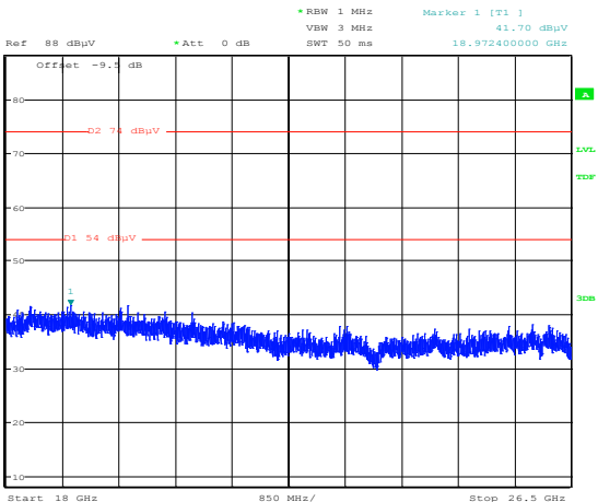
Figure 8.6-64: Radiated spurious emissions for BLE, mid channel, 18 to 26.5 GHz
