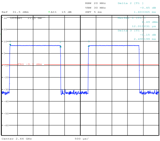
Figure 8.6-20: Pulse width for EV3
