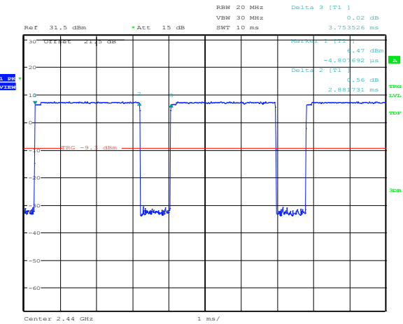
Figure 8.6-12: Pulse width for 2-DH3
