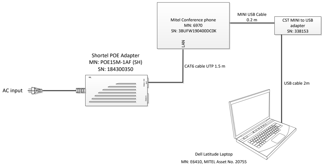
Figure 3.6-1: Setup diagram
