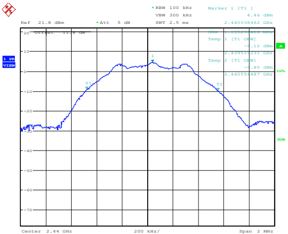
Figure 8.5-5: 99% occupied bandwidth – Mid channel
