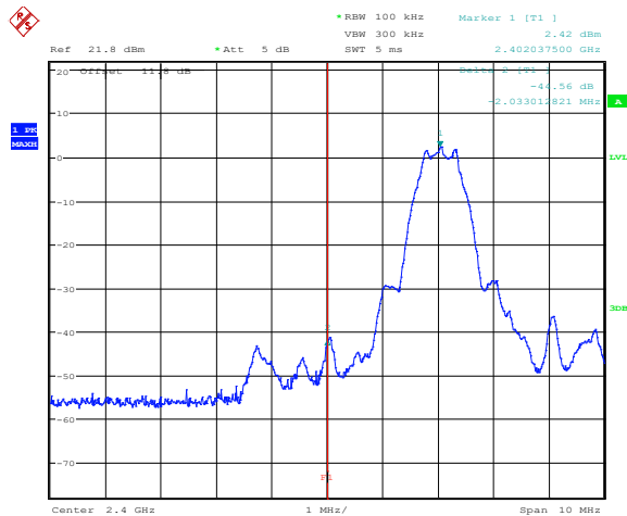
Figure 8.7-4: Conducted spurious (out-of-band) emissions, low channel – band edge
