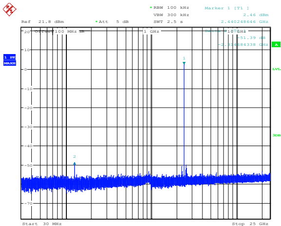
Figure 8.7-2: Conducted spurious (out-of-band) emissions, mid channel
