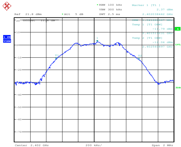
Figure 8.5-4: 99% occupied bandwidth – Low channel
