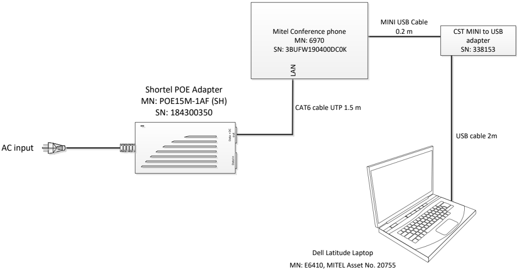
Figure 3.6-1: Setup diagram
