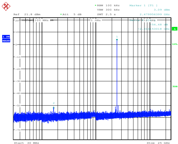
Figure 8.7-3: Conducted spurious (out-of-band) emissions, high channel
