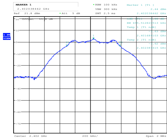
Figure 8.5-1: 6 dB bandwidth – Low channel
