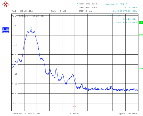
Figure 8.7-5: Conducted spurious (out-of-band) emissions, high channel – band edge
