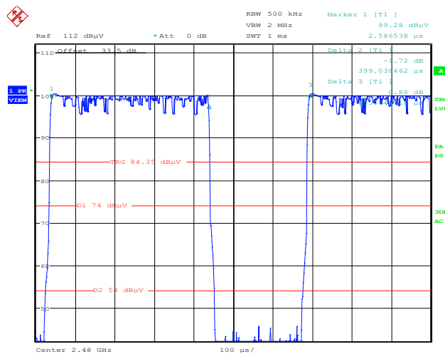
Figure 8.7-6: Transmission duration plot
