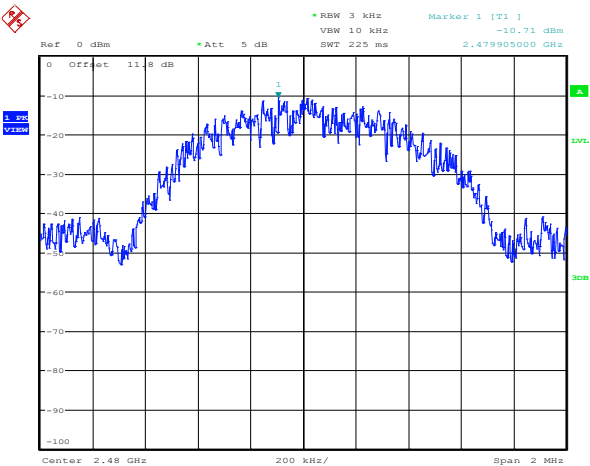
Figure 8.8-3: PSD High channel
