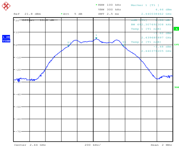
Figure 8.5-2: 6 dB bandwidth – Mid channel
