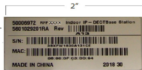
Product Label
