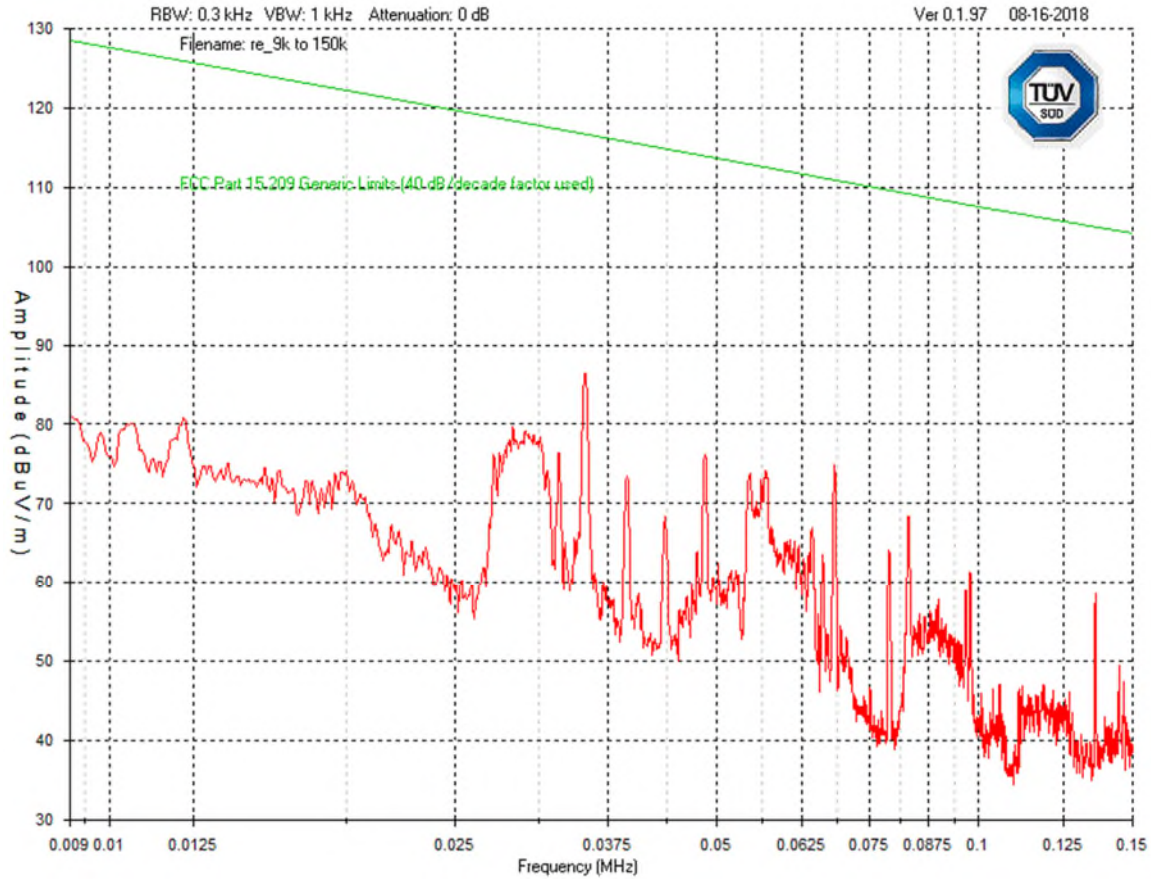
Peak Emissions Graph 9k to 150k
