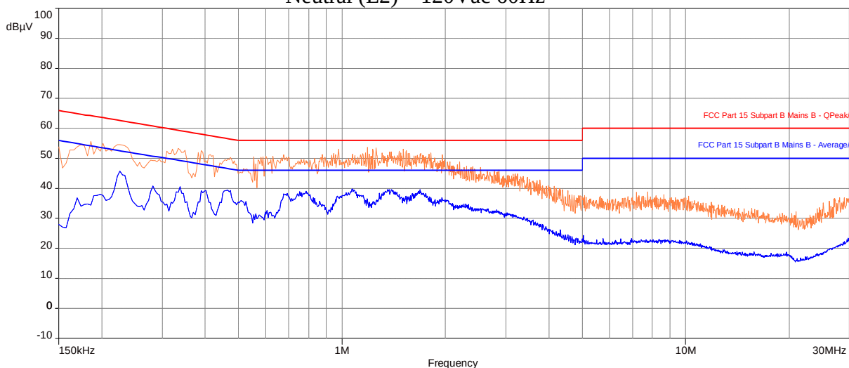
Neutral (L2) – 120Vac 60Hz
