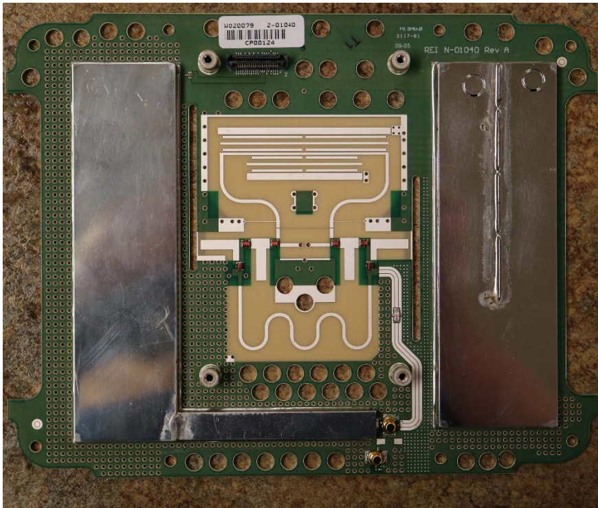
N-01040 RF Board – Side A (with shield):
