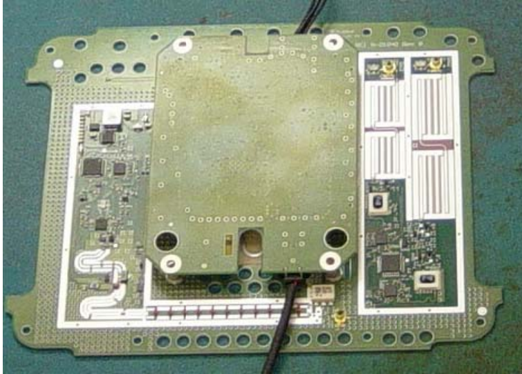
N-01040 RF Board – Side A (with shield):
