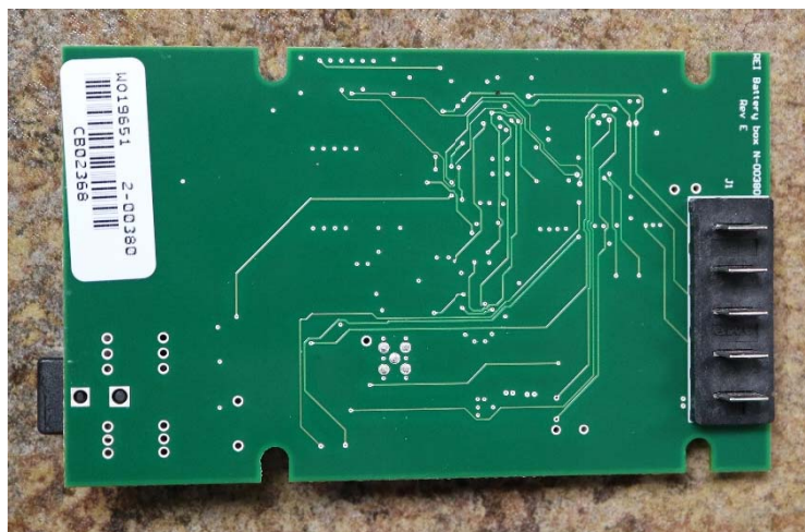
2-00380 ORION Battery board– Side A:
