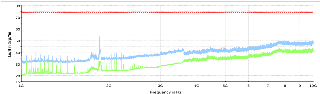
Figure 8.3-14: Cabinet Radiated spurious emissions 1 to 10 GHz, High channel
