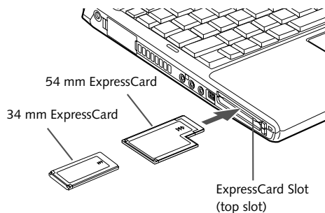
Figure 4-8. Installing/Removing ExpressCards
