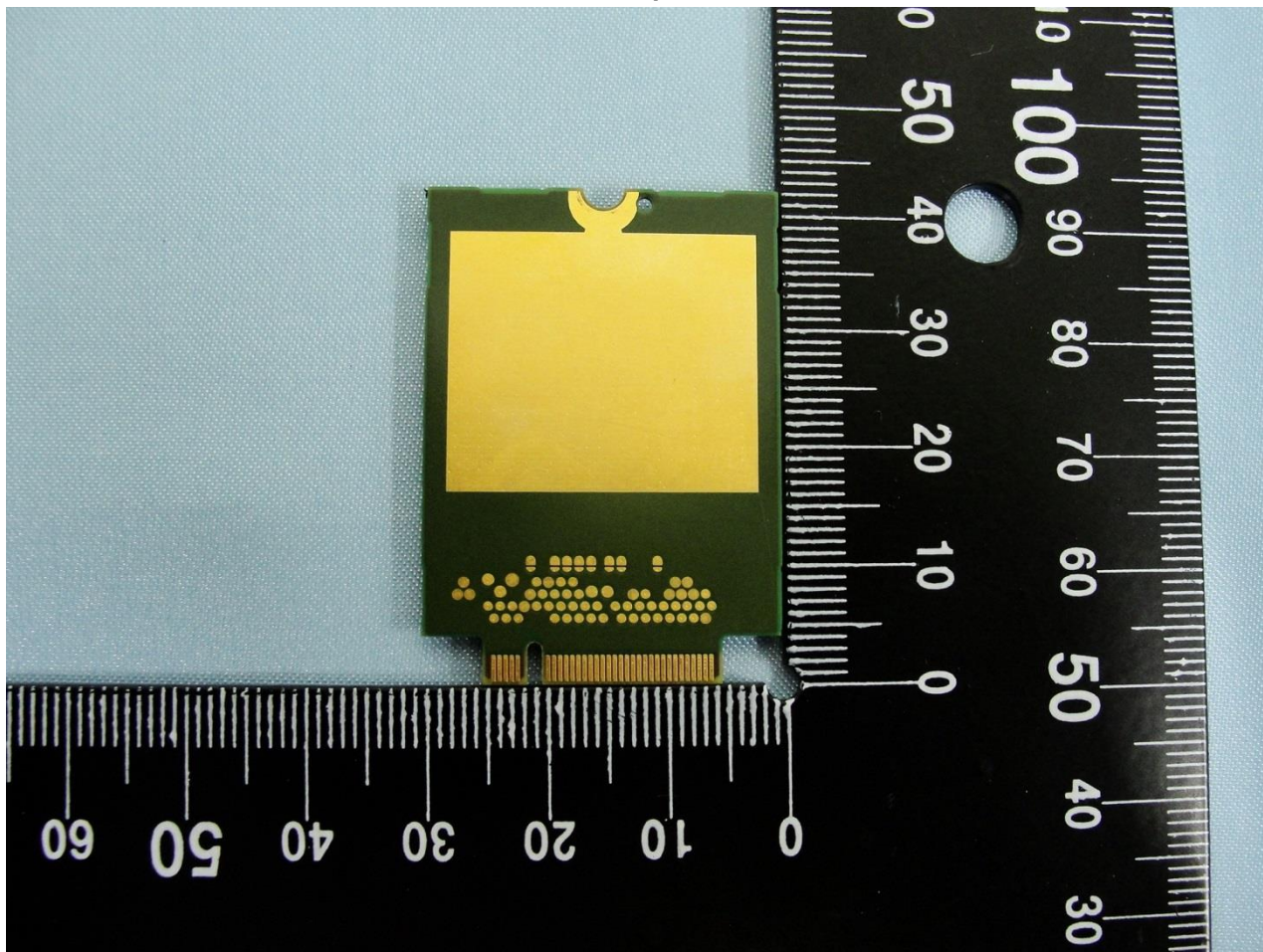
EUT: LTE module (Brand Name: AirPrime / Model Name: EM7355)
