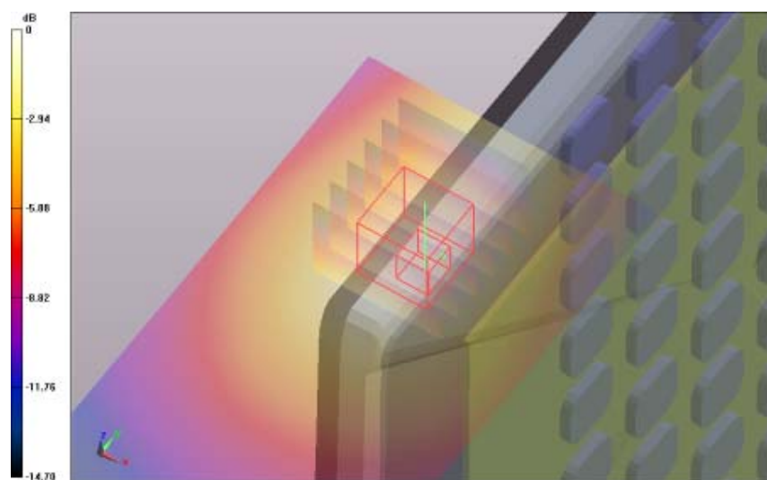
SAR Measurement Plot 86
