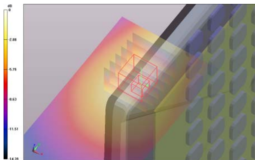
SAR Measurement Plot 85
