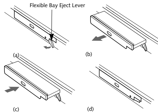
Figure 2-17 Removing/Installing a device in the Flexible Bay
