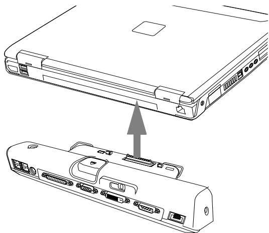
Figure 4-13. Attaching the Port Replicator
