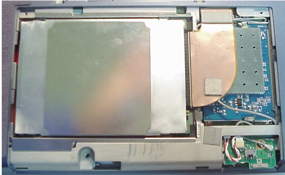
WLL4070 inside the Fujitsu Tablet Computer
