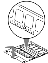
Figure 4-3. Installing a Second Memory Module
