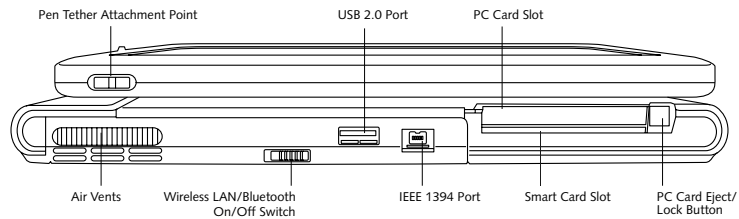
Figure 2-5. LifeBook T Series Tablet PC left-side panel
