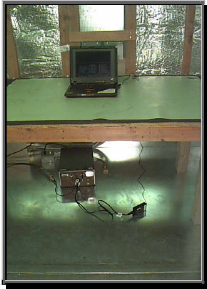
FCC Part 15.207 Conducted Emissions
