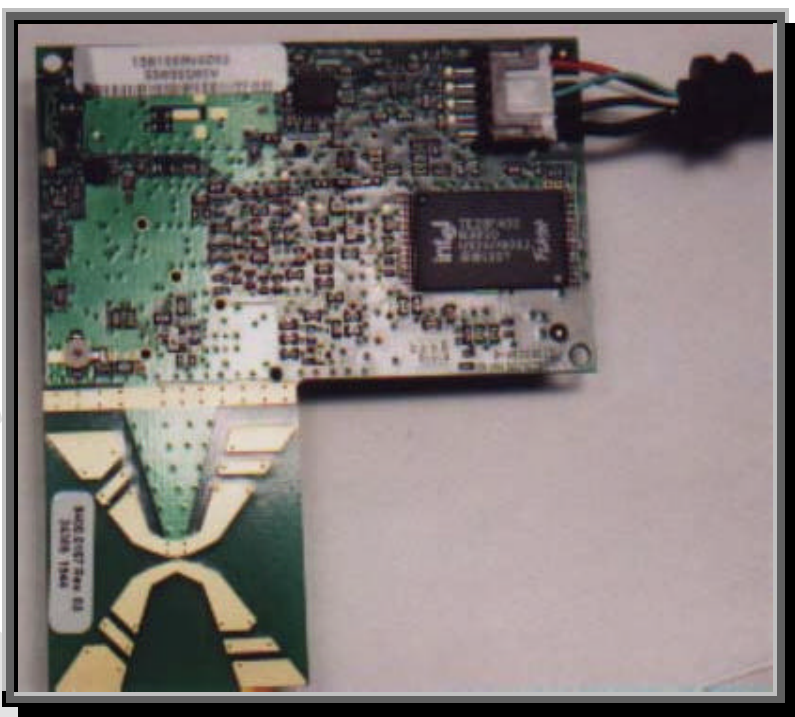
AnyPoint Module Backside
