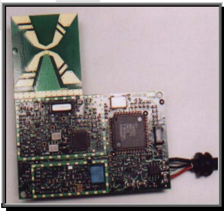
AnyPoint USB Module Front Without Shield (FRONT)
