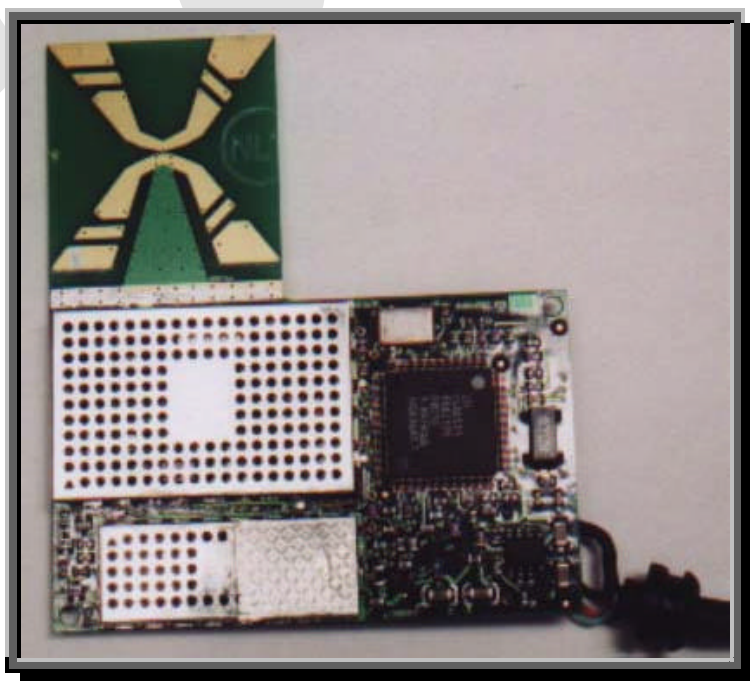
AnyPoint USB Module Close up (FRONT)
