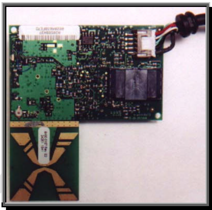
AnyPoint USB Module Close-up (BACK)
