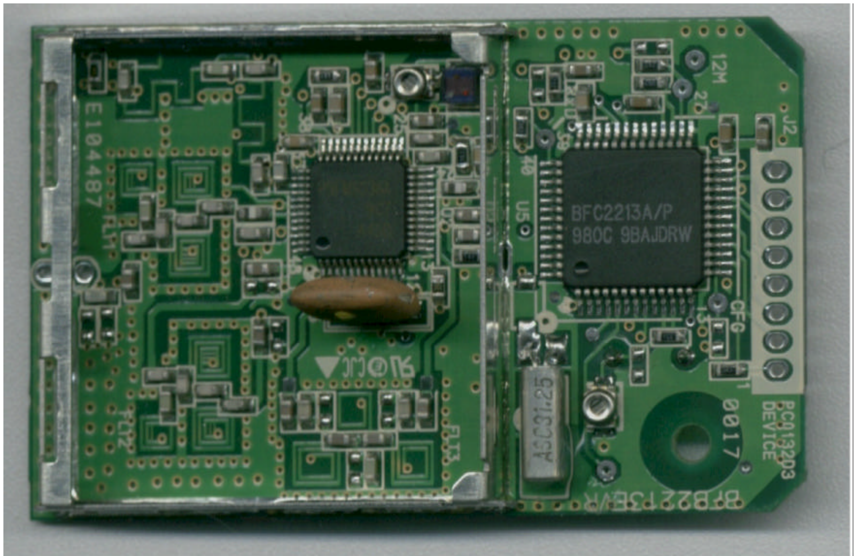
RF Module used in Keyboard, Mouse, and Gamepad - Component Side w/ RF Shield Removed
