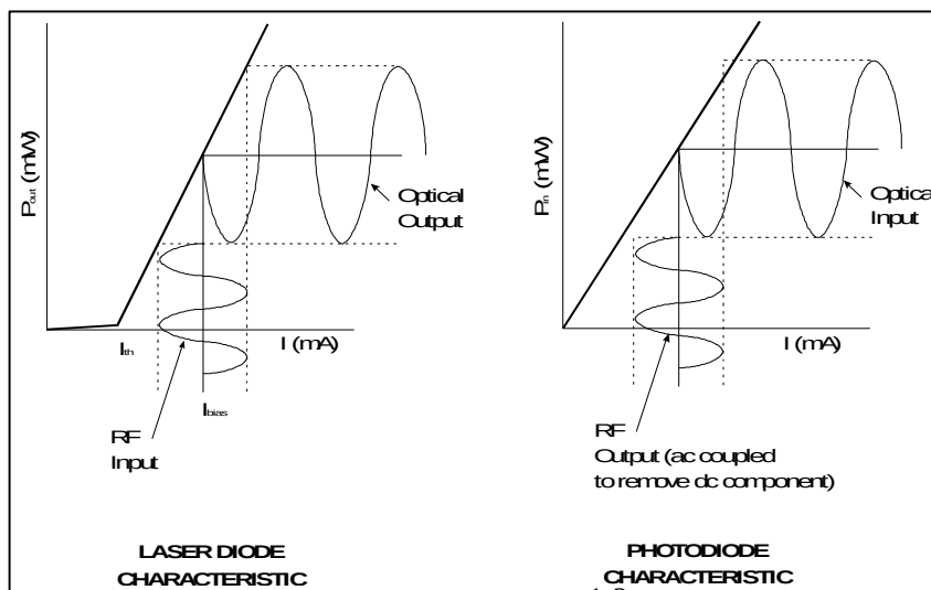
Figure 0. Laser diode and photodiode characteristics illustrating the
