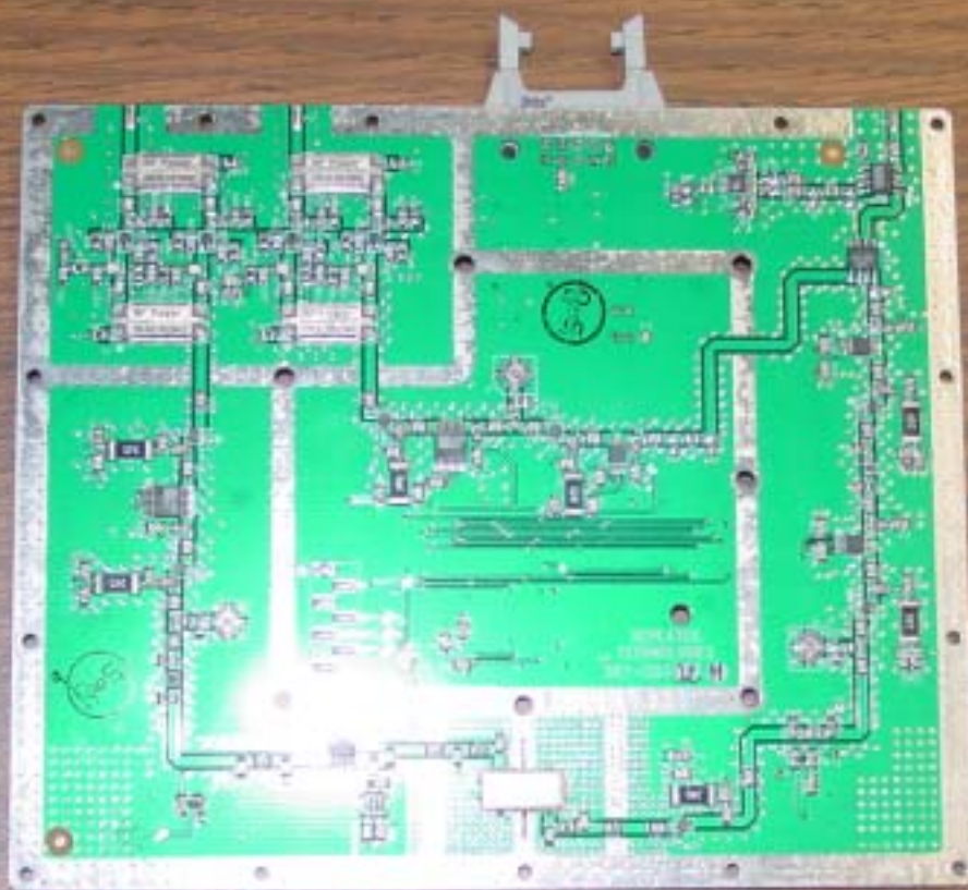
087-1303-01 Reverse Front End (Front) RF Module
