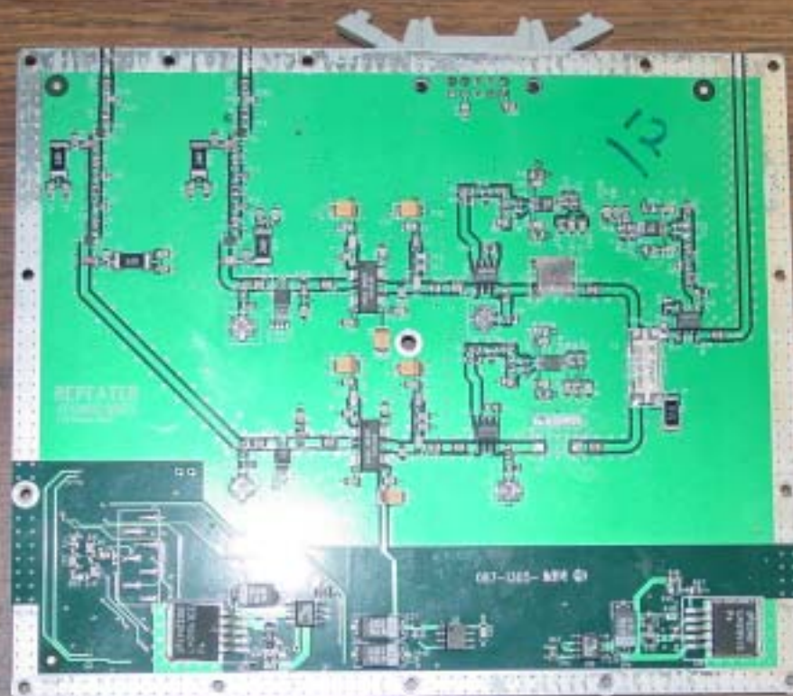
087-1304-04 Reverse Power Amp (Front) RF Module
