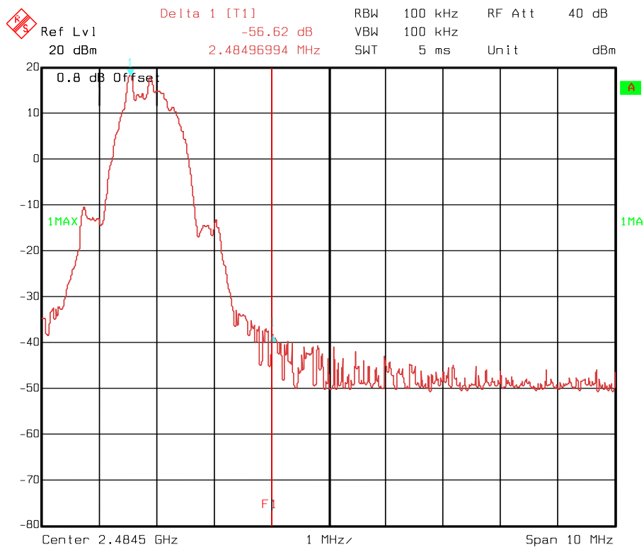
Band-edge conducted power ch 46, upper end
