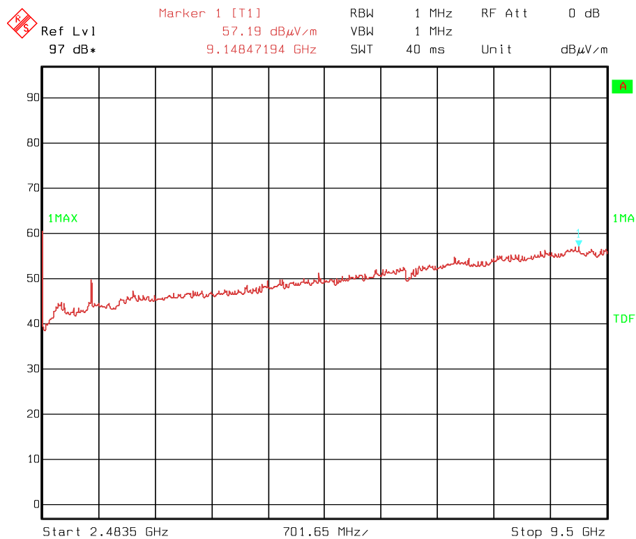
RF radiated emissions 2.4835-9.5 GHz channel 46
