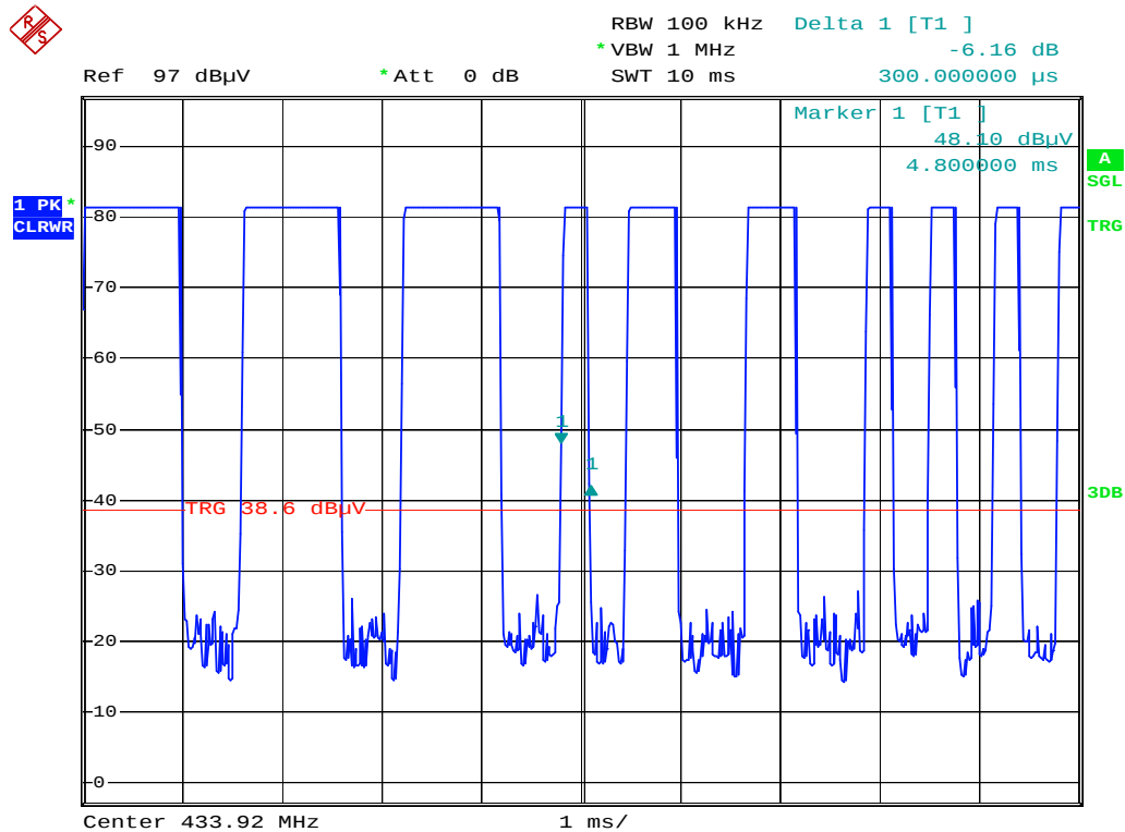
Time Slot 3
