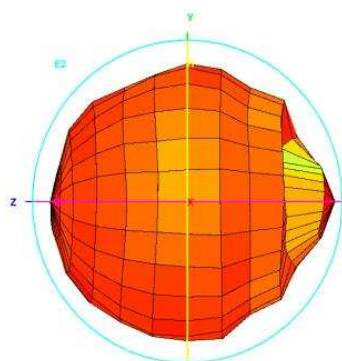
Total_3D_Left View_1.8GHz
