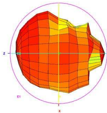
Total_3D_Left View_1.8GHz
