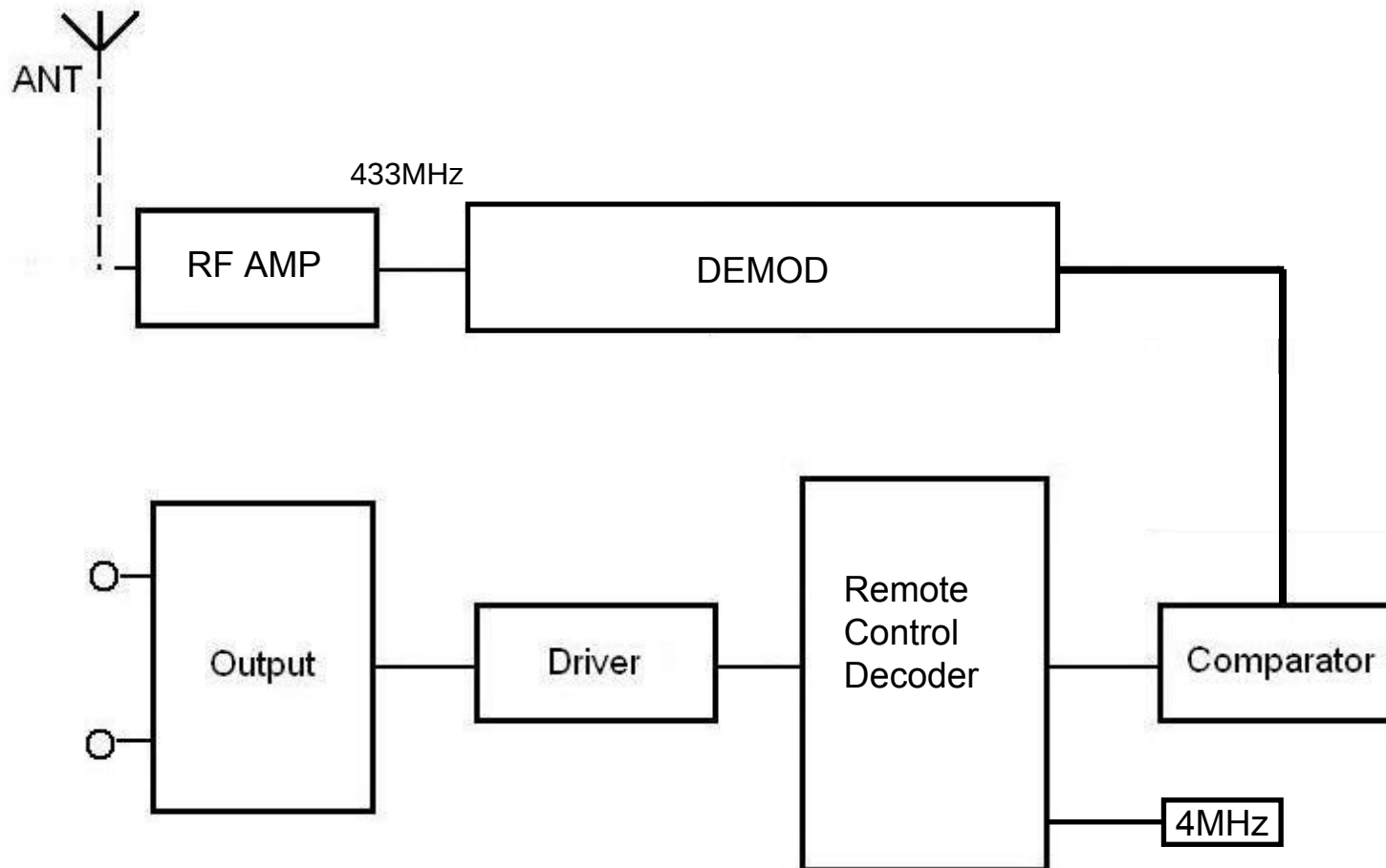
3-Stage On/Off Remote - Operational Block Diagram (Receiver)
