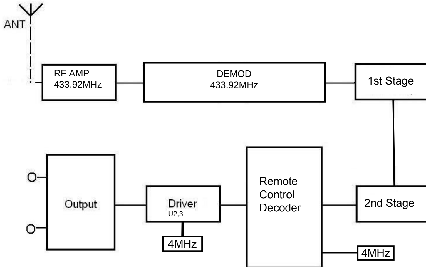
Full Featured Remote - Operational Block Diagram (Receiver)
