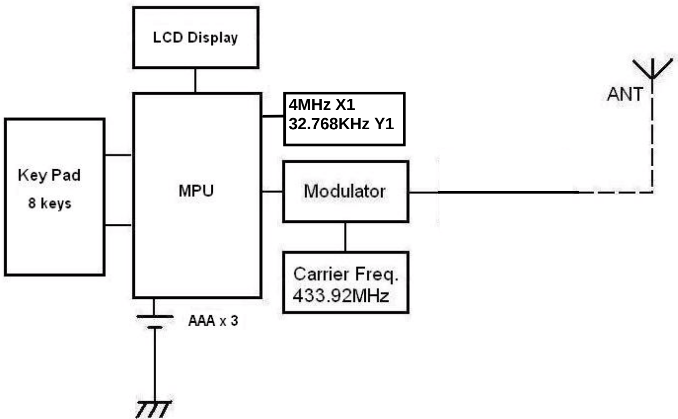
Full Featured Remote (Transmitter) - Operational Block
