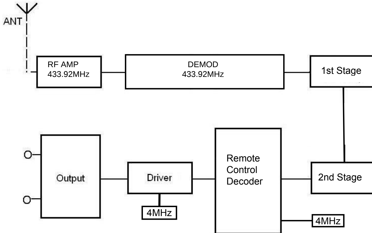
Mid Line Remote - Operational Block Diagram (Receiver)
