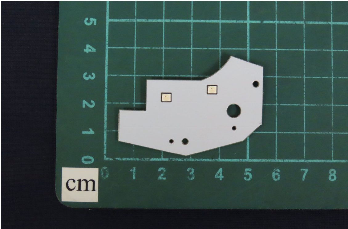
(7) EUT Photo
