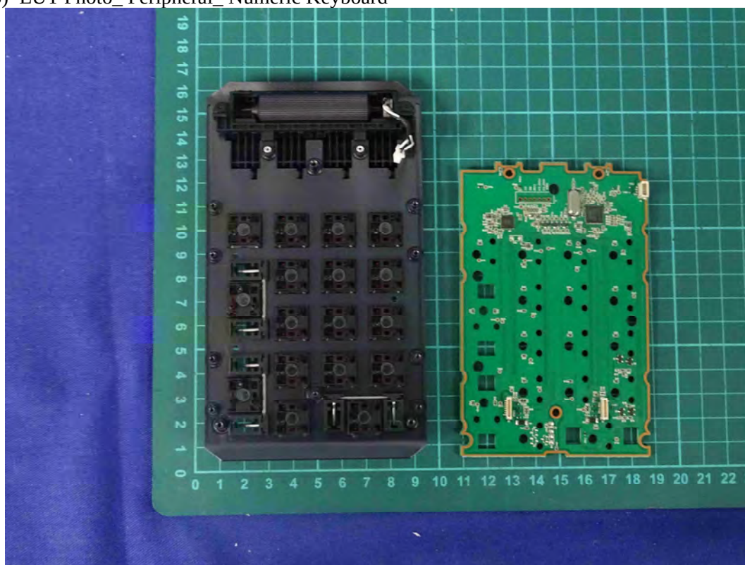
(46) EUT Photo_ Peripheral_ Numeric Keyboard
