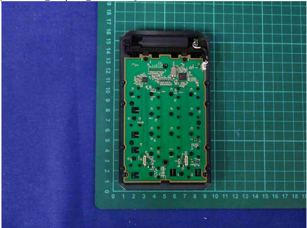
(44) EUT Photo_Peripheral_Numeric Keyboard
