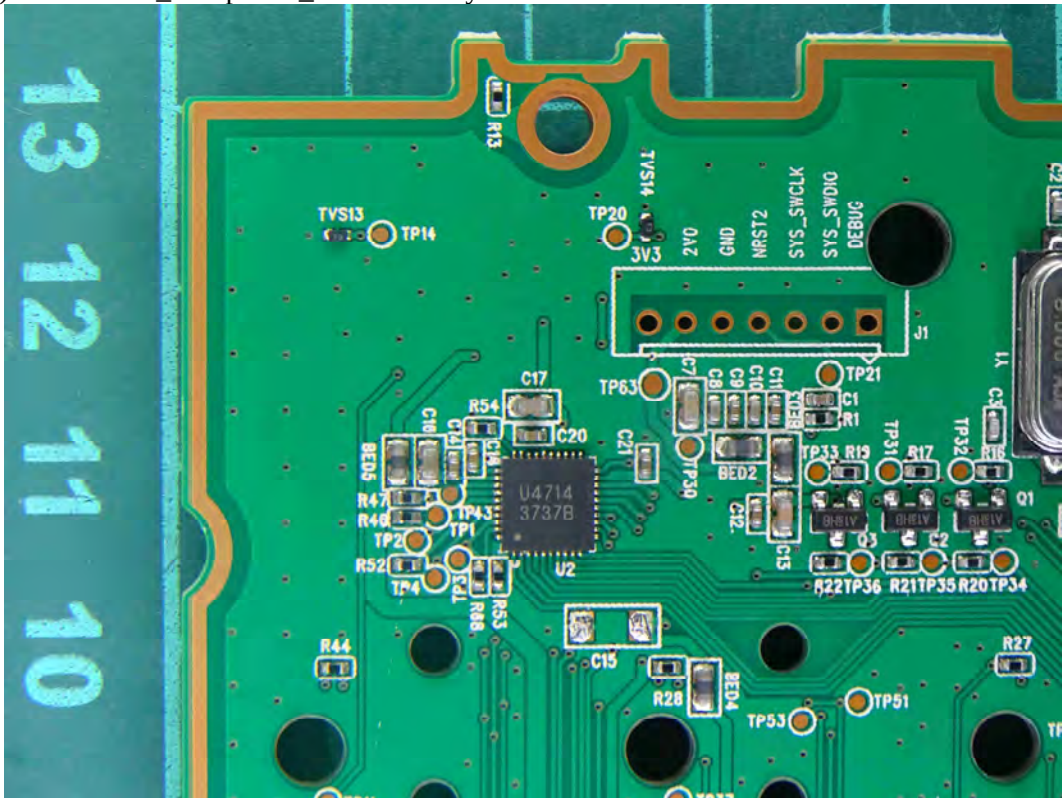
(48) EUT Photo_ Peripheral_ Numeric Keyboard
