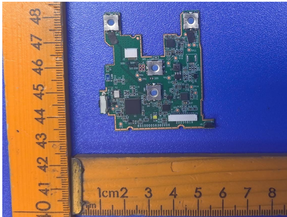
Figure 11: Main board view_1 of EUT
