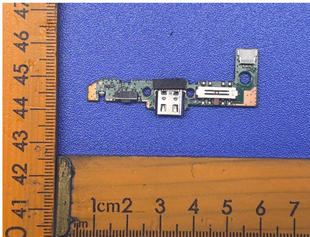
Figure 14: USB Charging board view_2
