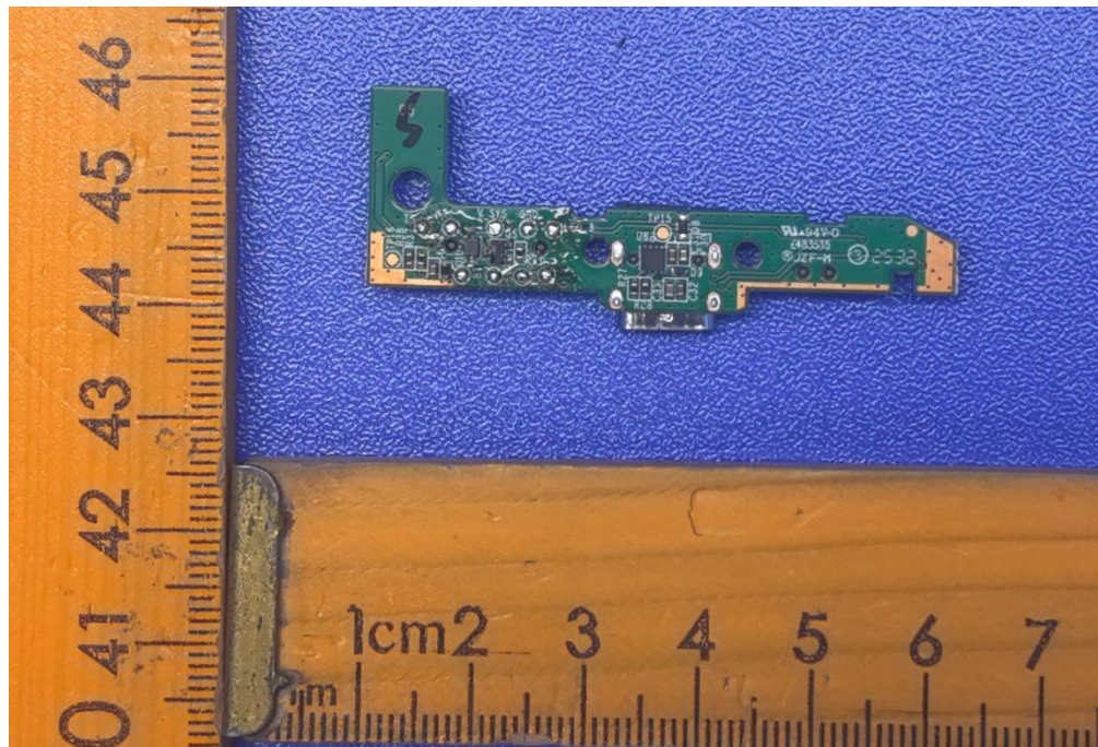
Figure 13: USB Charging board view_1
