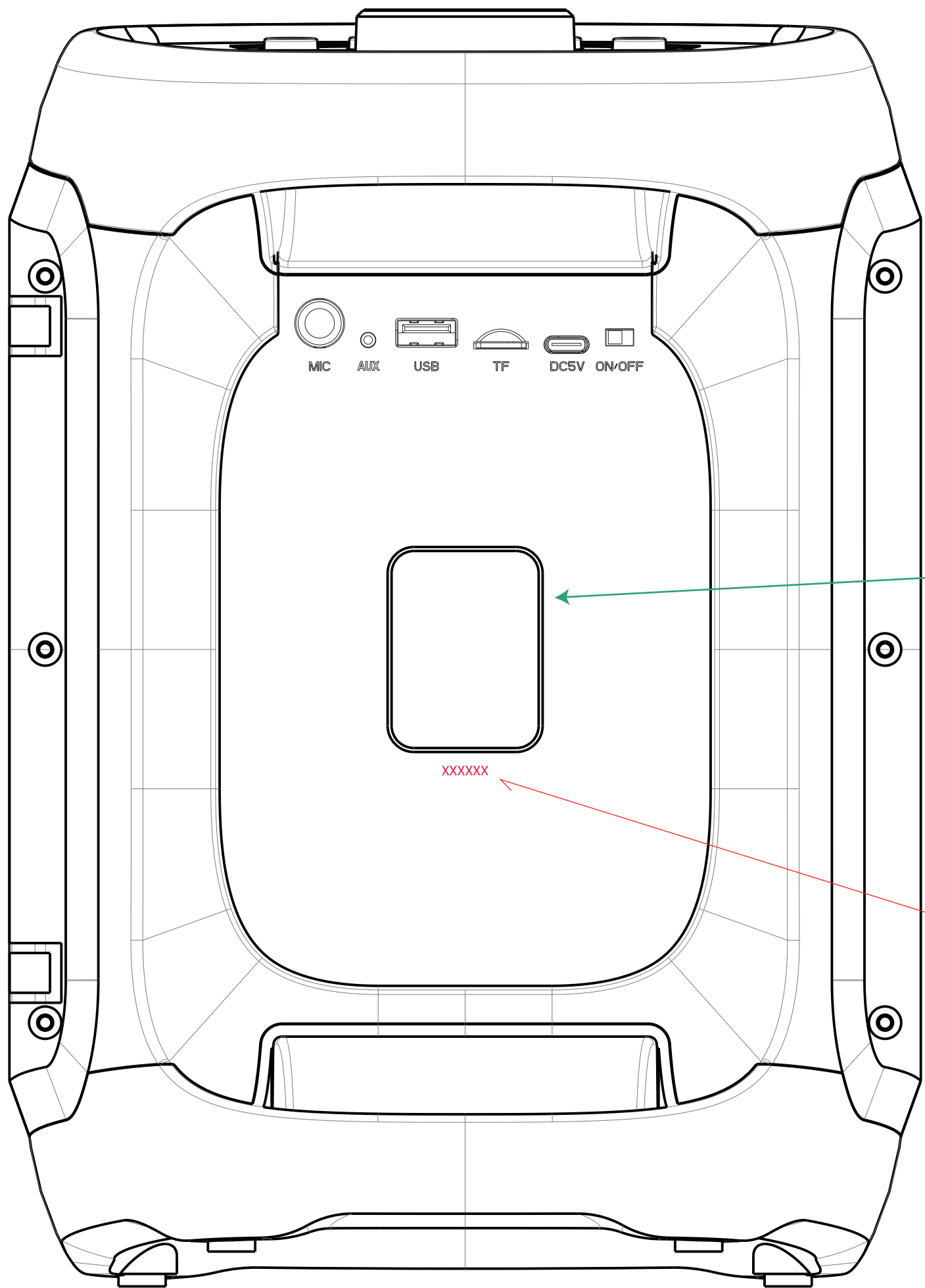
Date Code Laser etching Font size: 7pt (Font height: 2mm)
