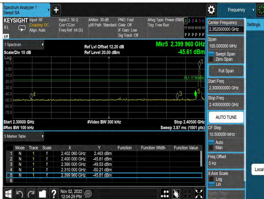
DH5-Ant1-Low-2402-2.46
