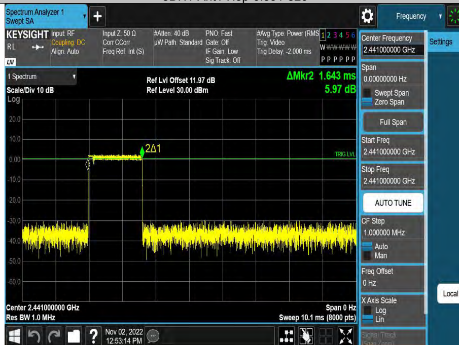
3DH3-Ant1-Hop-1.643-160
