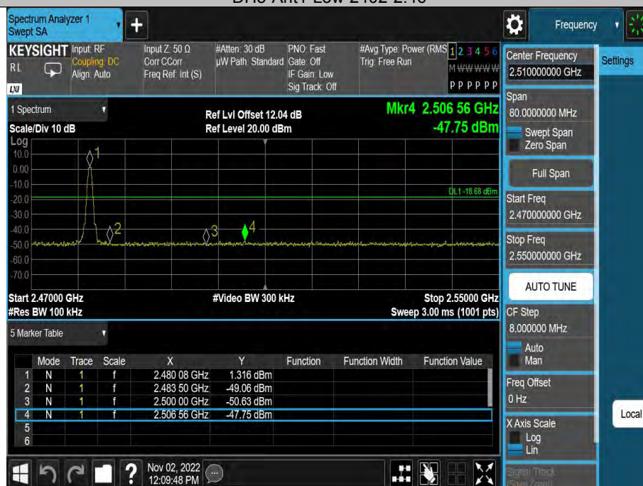
DH5-Ant1-High-2480-1.32
