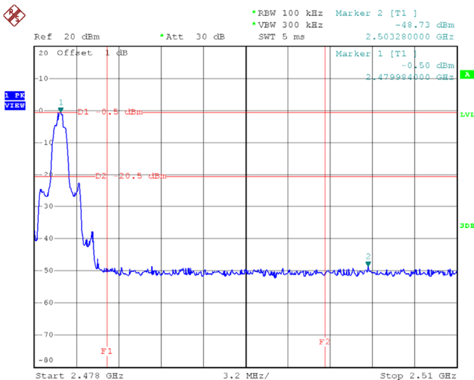
High Band Edge Plot on channel 78 @8-DPSK
