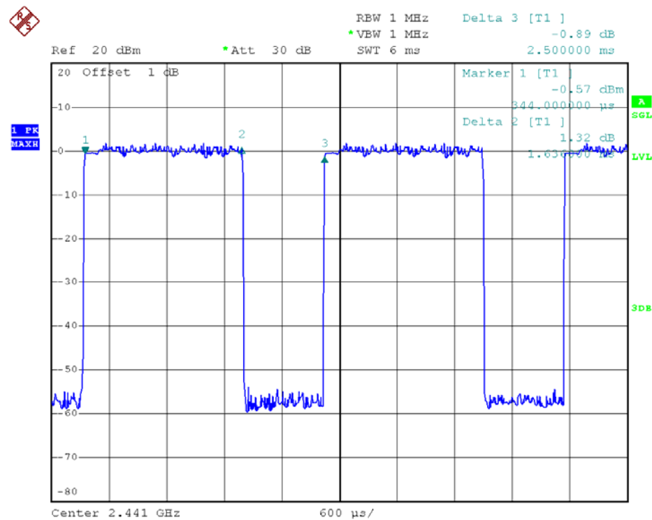
39 Channel @ 3DH3
