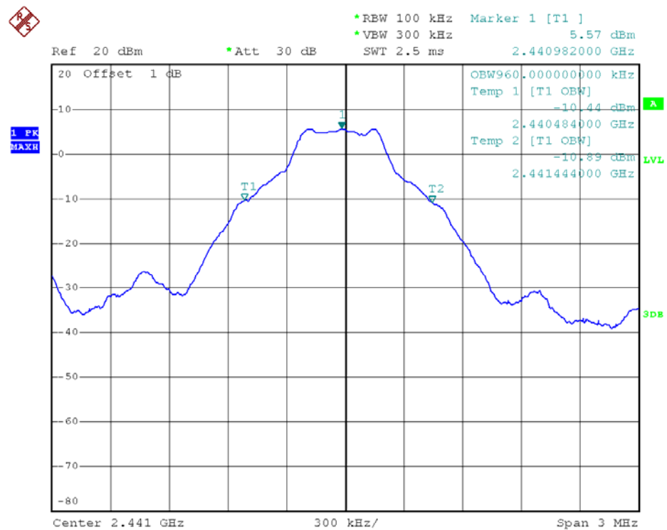
39 Channel @ GFSK
