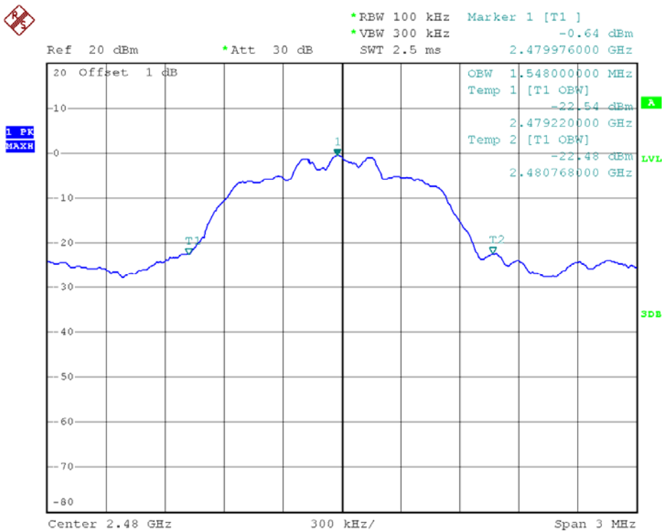
78 Channel @ \pi/4 -DQPSK
