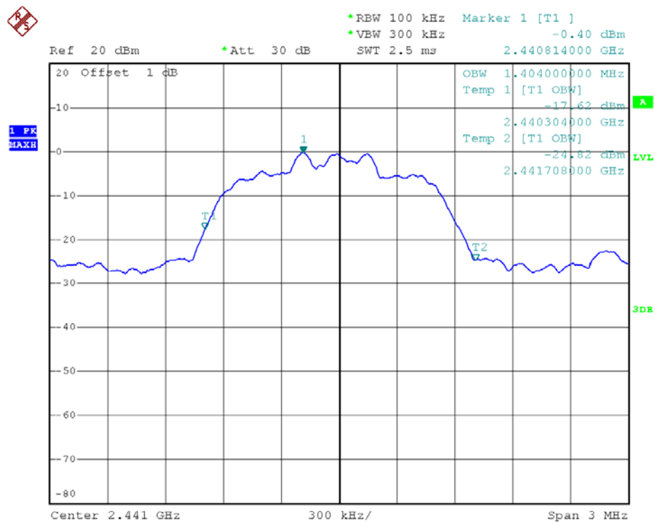
39 Channel @ 8-DPSK
