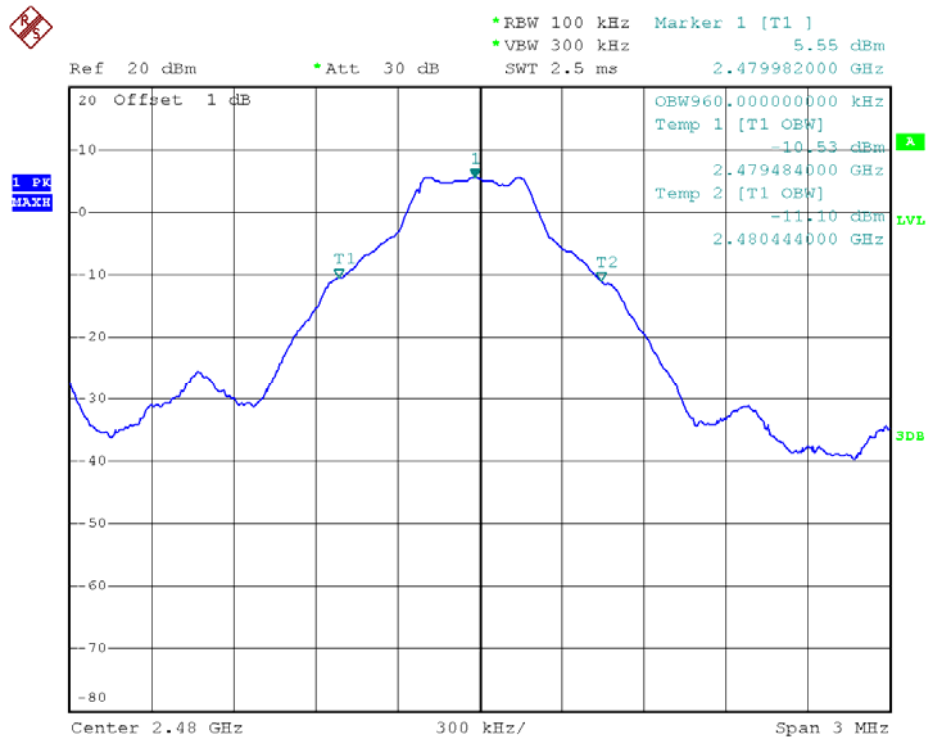
78 Channel @ GFSK
