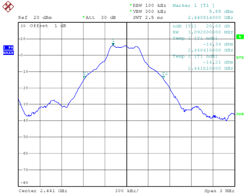
39 Channel @ GFSK
