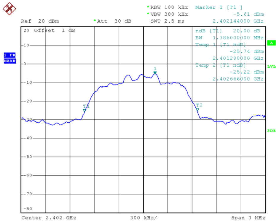
0 Channel @ 8-DPSK
