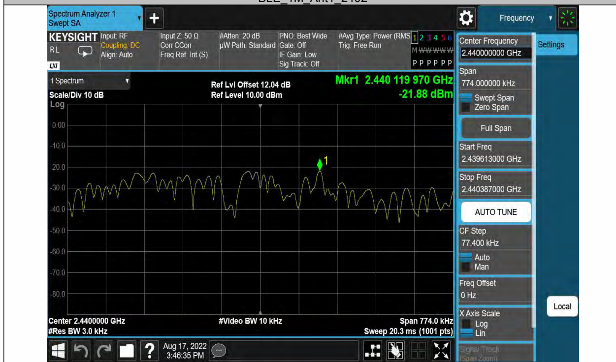
BLE_1M_Ant1_2440
