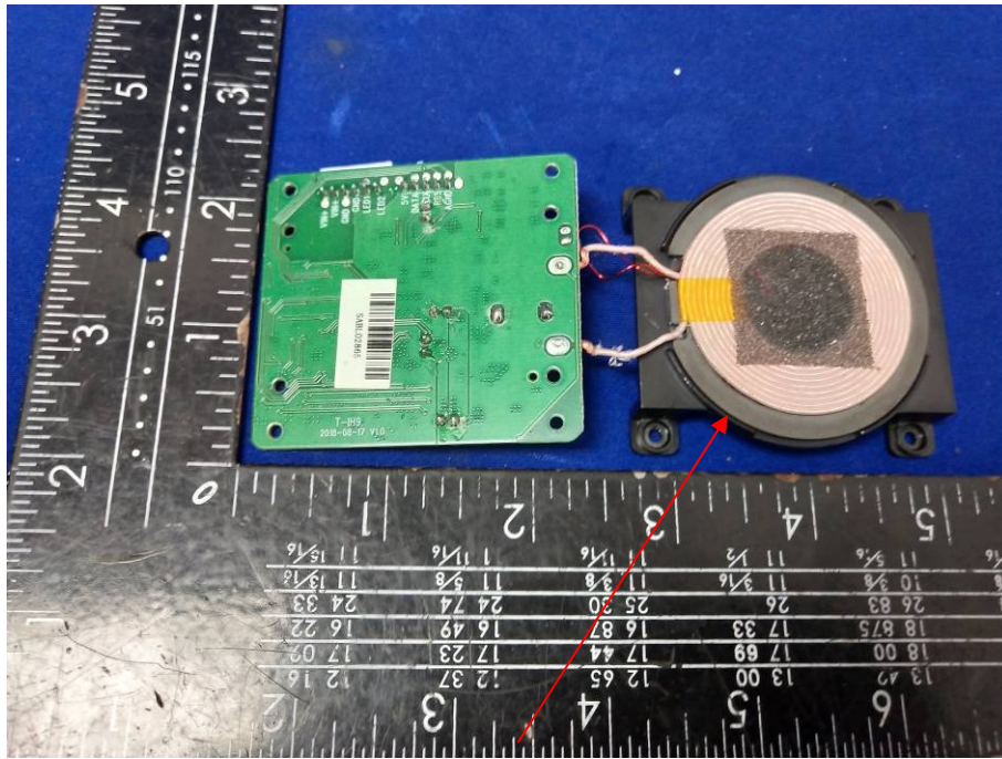
WPT Coil
